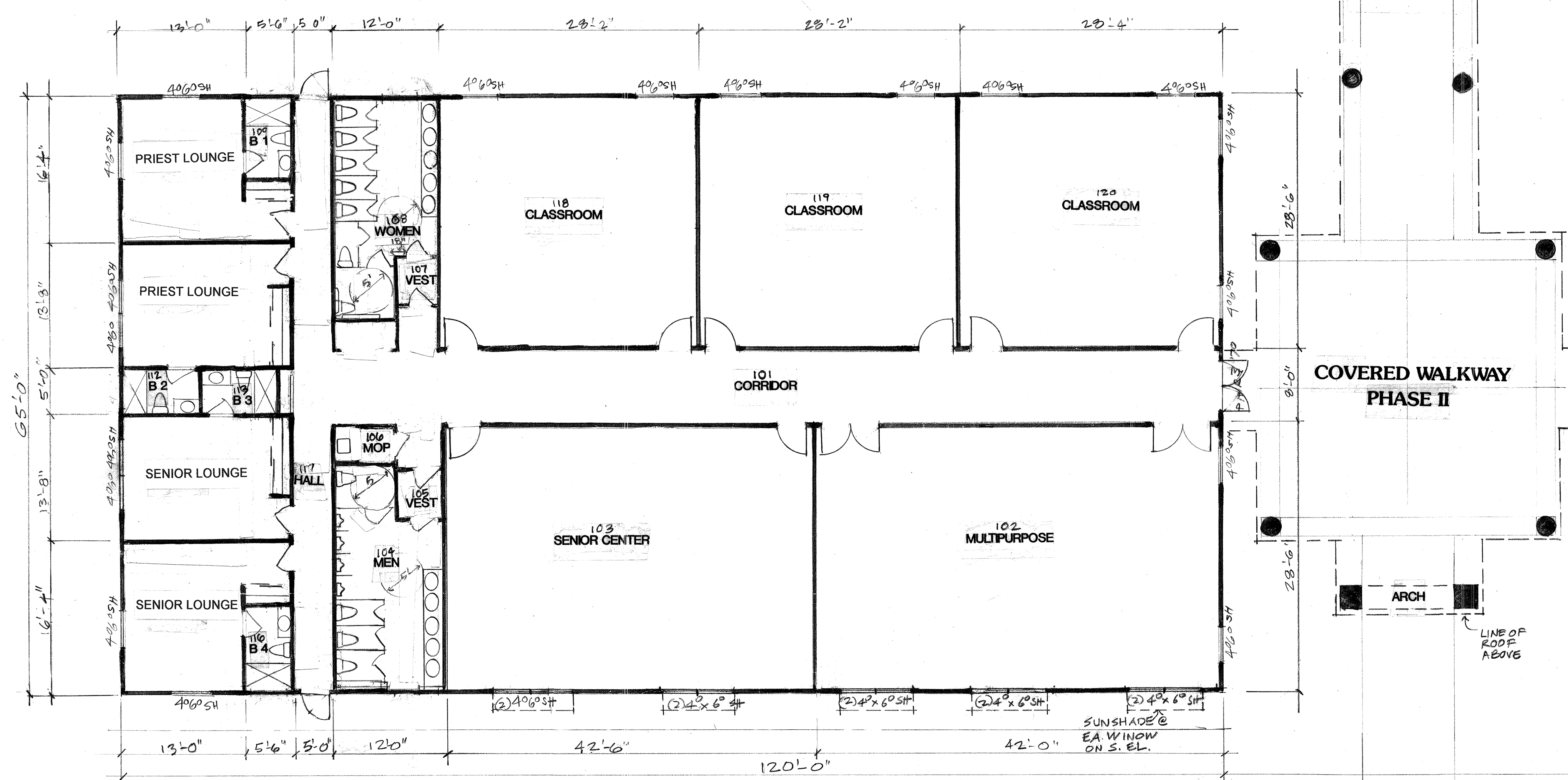
BUILDING D - PHASE II PROPOSED FLOOR PLAN 7800 sq NORTH SCALE = 1/8" = 1'-0" 0 5 10 20 40
